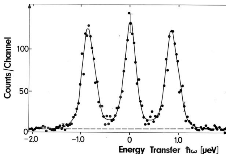
Fig.7 Hyperfine splitting in cobalt at room temperature. The spectrum obtained on the BSS IN10 was published in Z.Physik B20 , 385-389 (1975)
