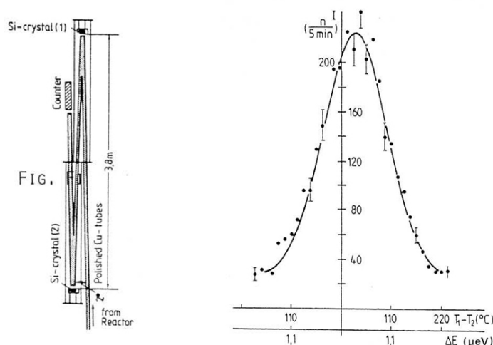
Fig.3a The first BS setup on a vertical tube at the FRM (1964)
